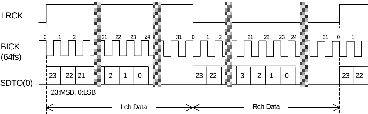
Figure 7. Mode 4, 6 Timing
