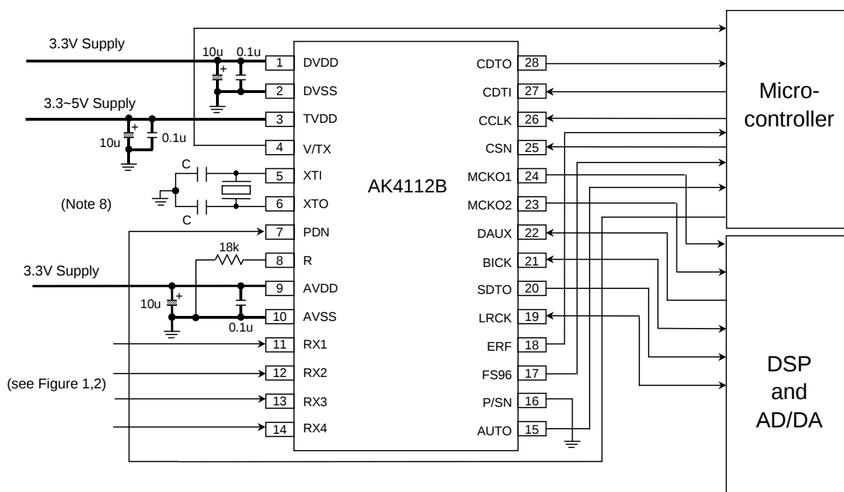
Figure 11. Typical Connection Diagram (Serial Mode)
