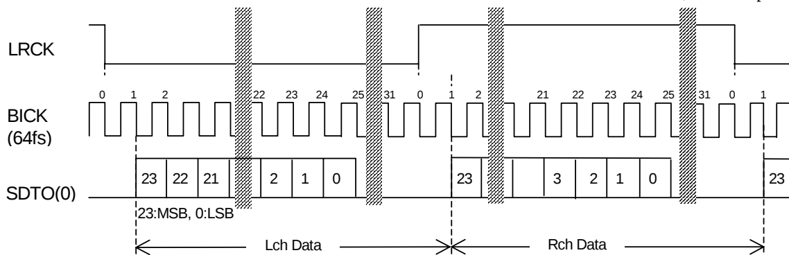
Figure 8. Mode 5, 7 Timing
