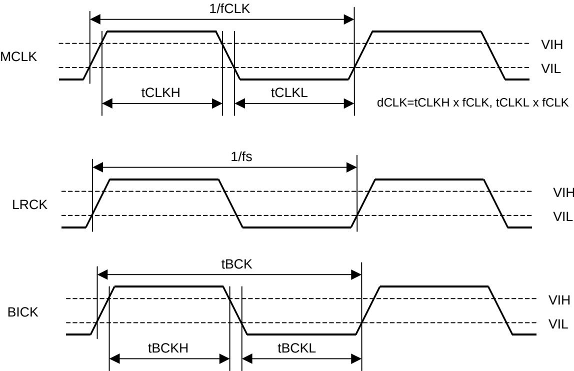
Figure 3. Clock Timing
