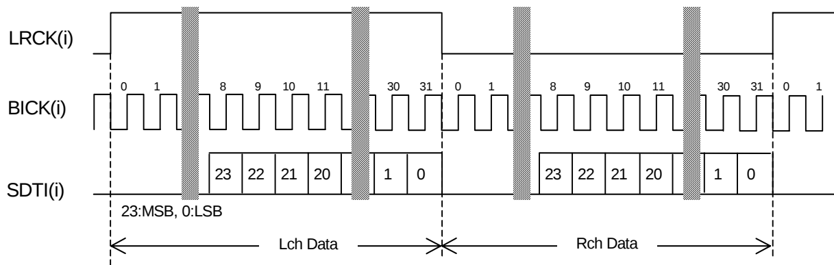
Figure 11. Mode 3 Timing
