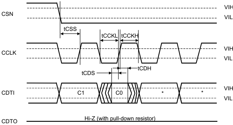
WRITE/READ Command Input Timing
