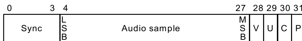
Figure 14. Sub-frame format
