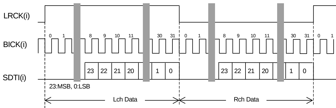
Figure 11. Mode 3 Timing
