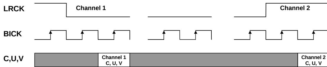
Figure 7. Audio routing, DIF modes 5 and 7 (I²S)
