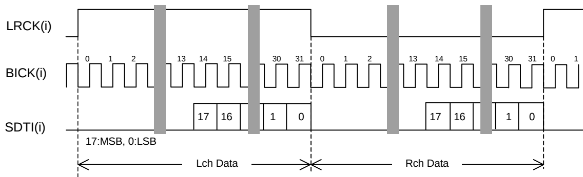
Figure 9. Mode 1 Timing
