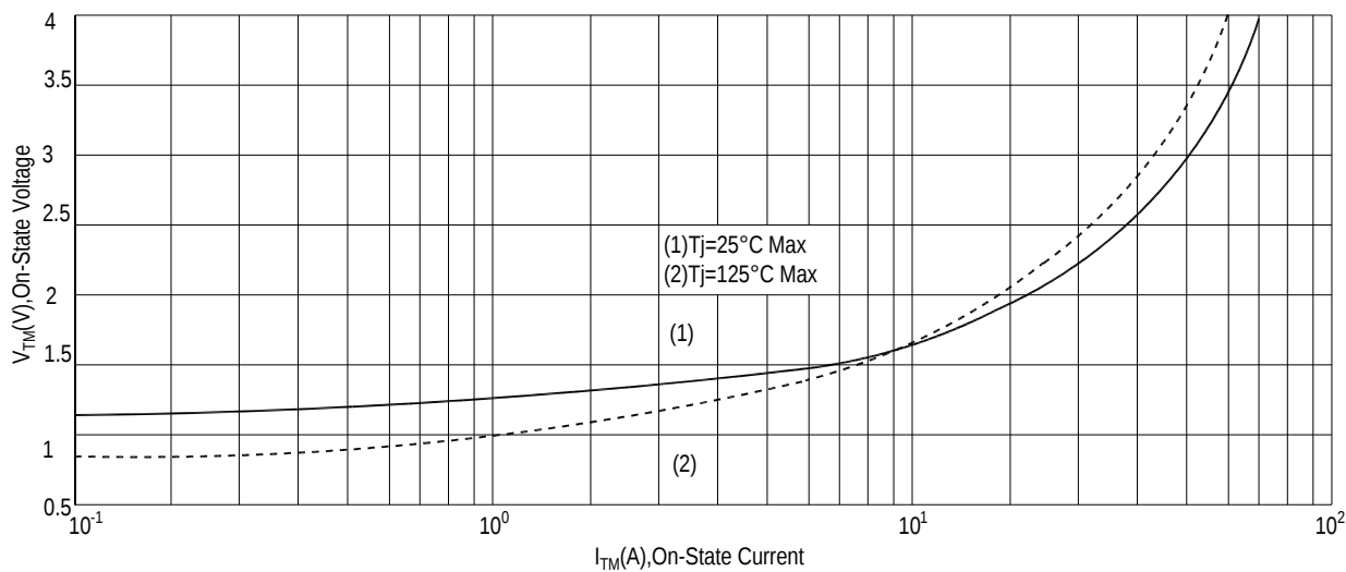
FIG.9: On-state characteristics(Max)
