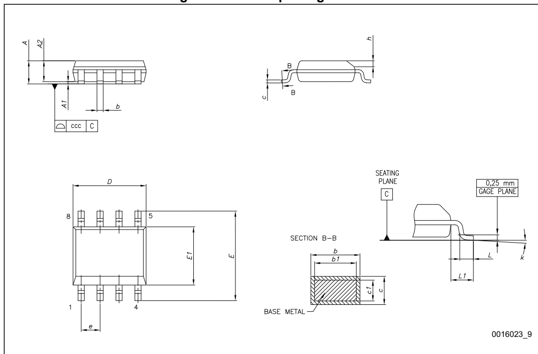
Figure 28. SOIC8 package outline
