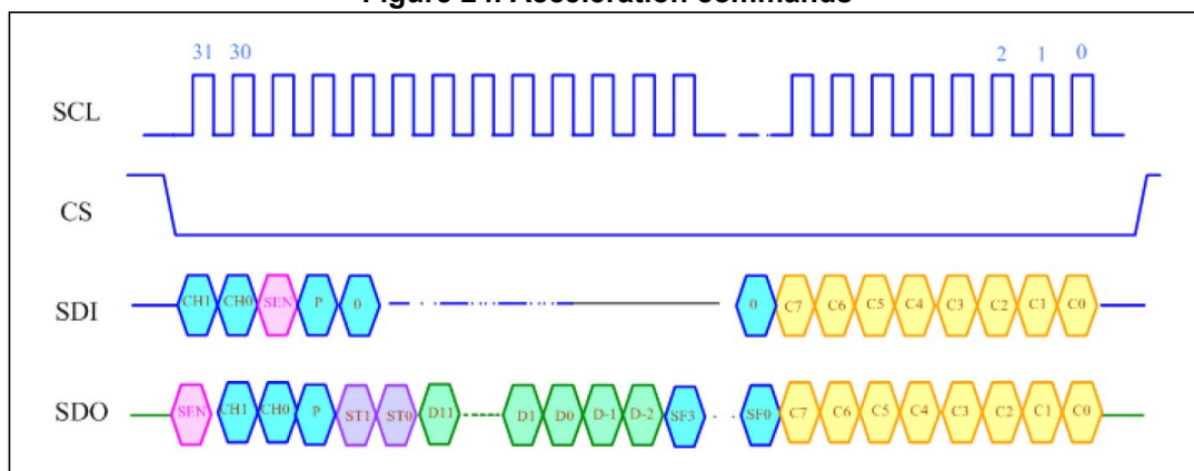
Figure 24. Acceleration commands
