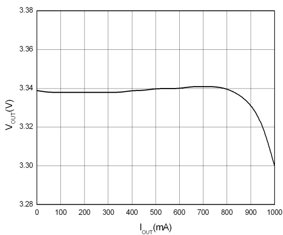
Fig.12 Load Regulation V_{IN} = 3.6V V_{OUT} = 3.3V (PWM Mode)
