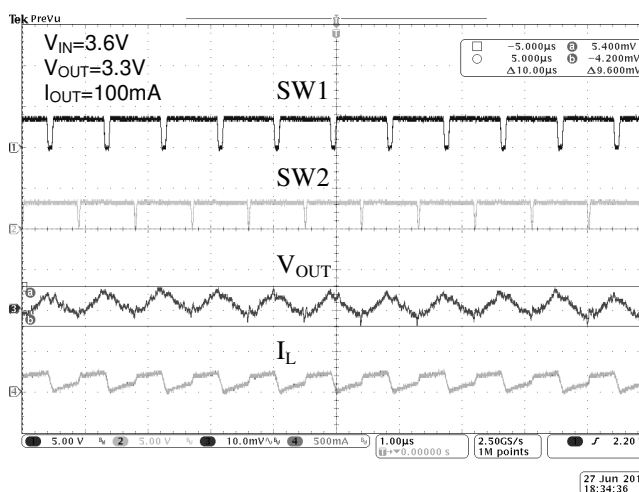
Fig.18 Buck-Boost Operation
