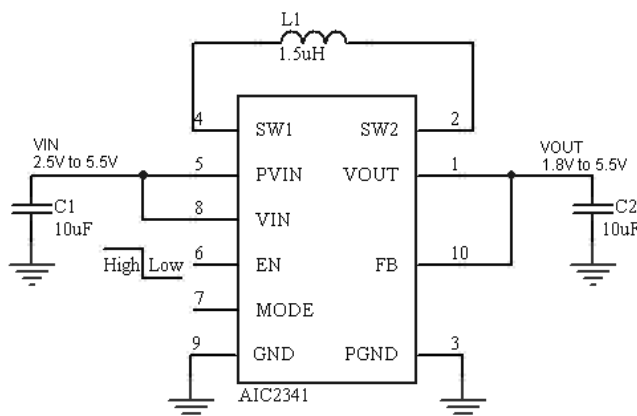
Fig.1 Application Circuit
