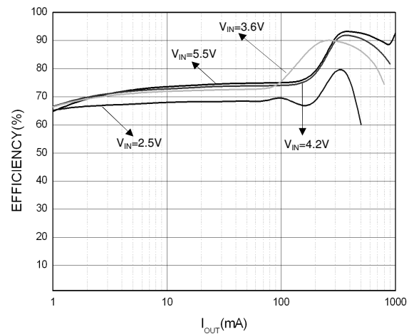
Fig.9 Efficiency vs. Output Current V_{OUT} = 5V (PSM Mode)
