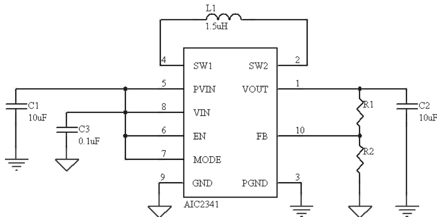
Fig.26 Adjustable Output Voltage
