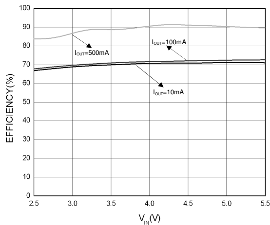
Fig.10 Efficiency vs. Input Voltage V_{OUT} = 3.3V (PSM Mode)
