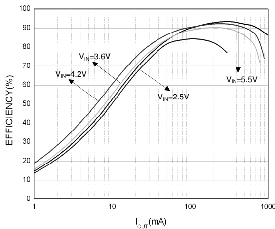
Fig.8 Efficiency vs. Output Current V_{OUT} = 5V (PWM Mode)
