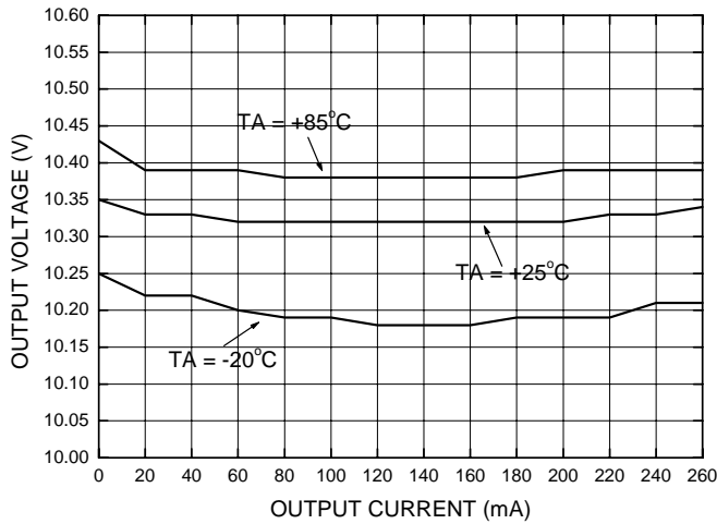
Fig. 5 Load regulation
