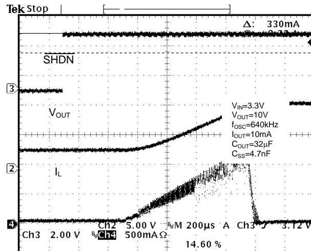
Fig. 10 Startup waveform with soft-start
