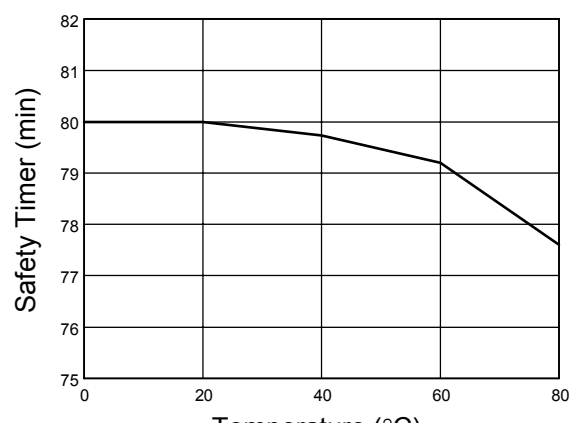
Fig.5 Safety Timer vs. Temperature
