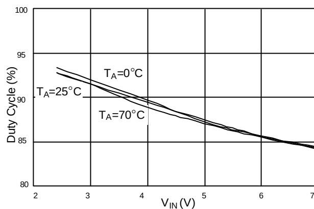
Fig. 4 Duty Cycle vs. V_{\text{IN}} Voltage
