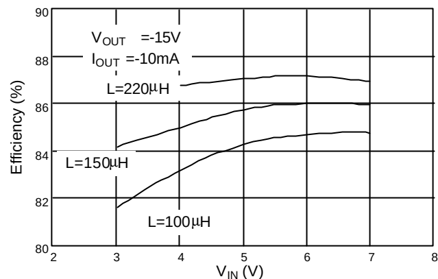
Fig. 6 Efficiency vs. V_{IN}
