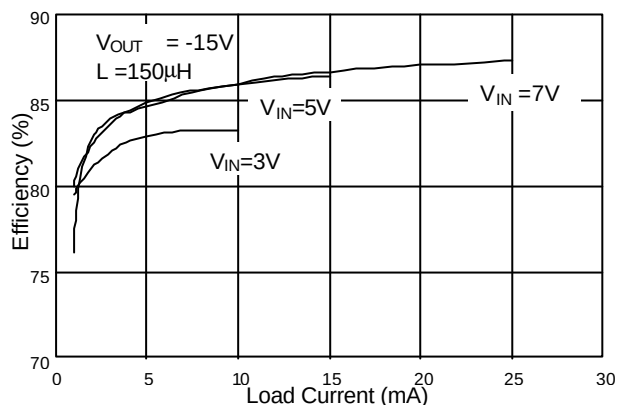
Fig. 5 Efficiency vs. Load Current
