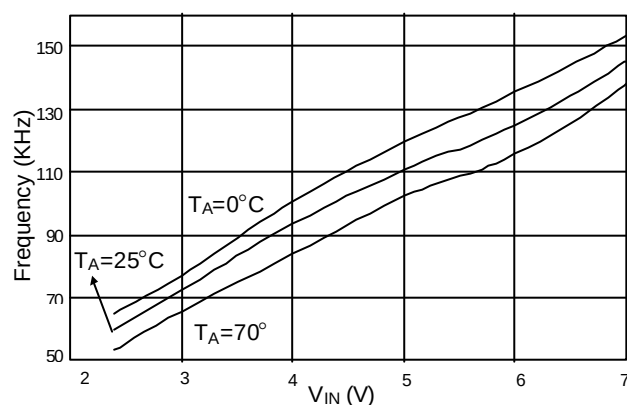
Fig. 3 Frequency vs. V_{\text{IN}} Voltage
