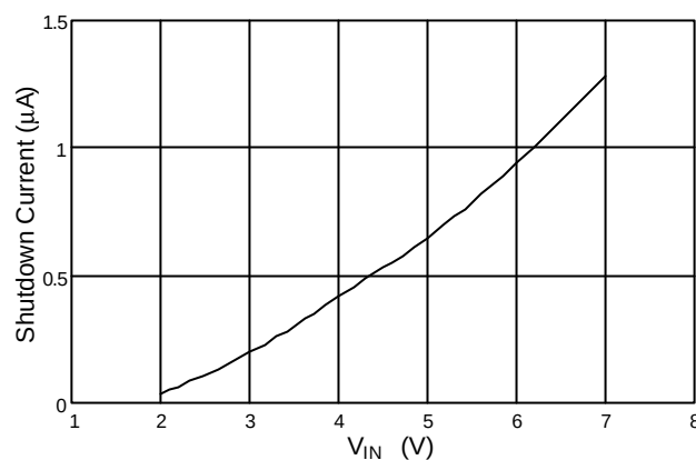
Fig. 2 Shutdown Current vs. V_{\text{IN}}
