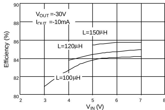
Fig. 10 Efficiency vs. V_{IN}
