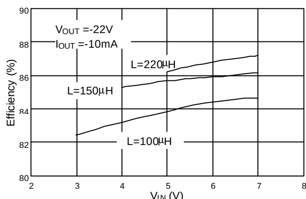
Fig. 8 Efficiency vs. V_{IN}
