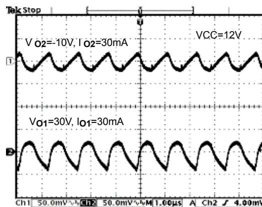
Fig 4. Ripple Voltage Waveforms
