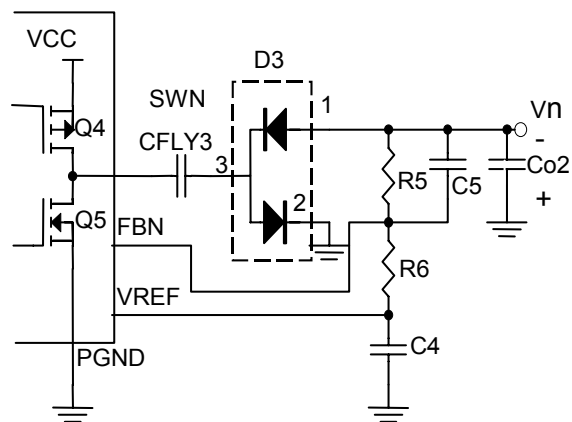
Fig. 17 Structure of Negative Charge Pump
