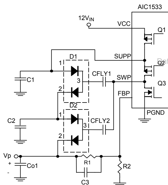
Fig.16 Structure of Positive Charge Pump
