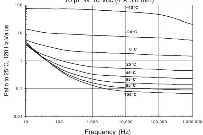
Impedance vs. Temperature & Frequency 10 \mu F @ 16 Vdc (4 X 5.8 mm)
