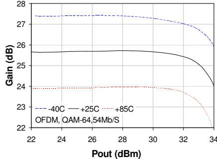
Gain vs Pout vs Temperature (Freq = 3.5 GHz, Vcc=5V)
