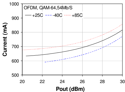
Current vs Pout vs Temperature (Freq = 3.5 GHz, Vcc=5V)
