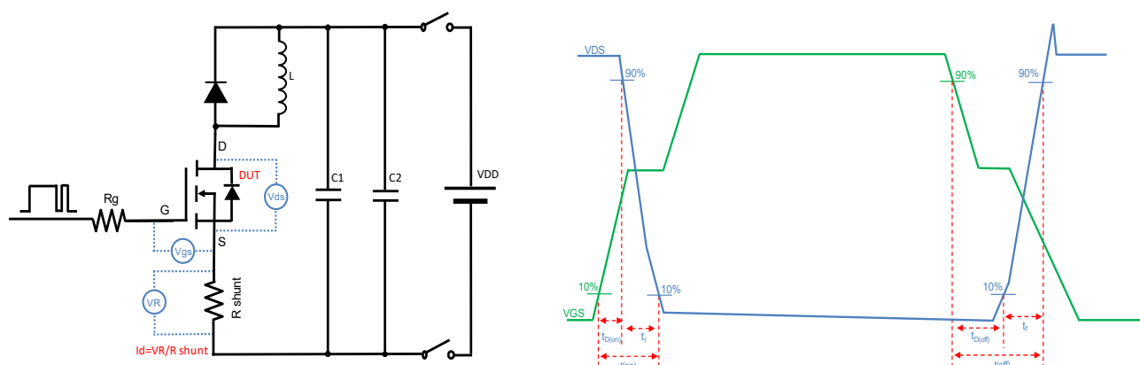
Figure C. Resistive Switching Test Circuit &amp; Waveform
