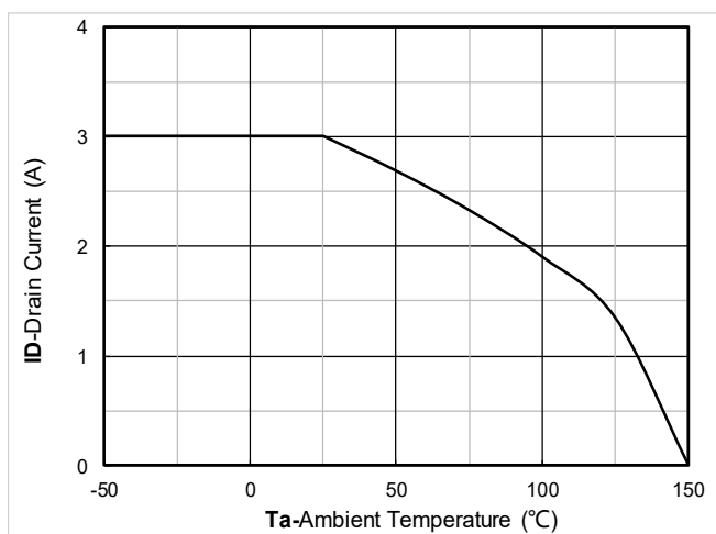
Figure 11. Current dissipation
