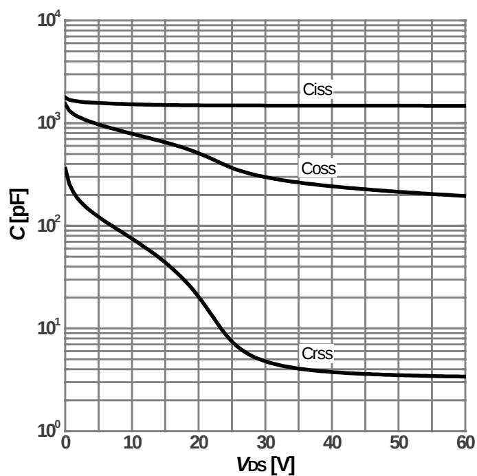
Diagram 13: Typ. capacitances
