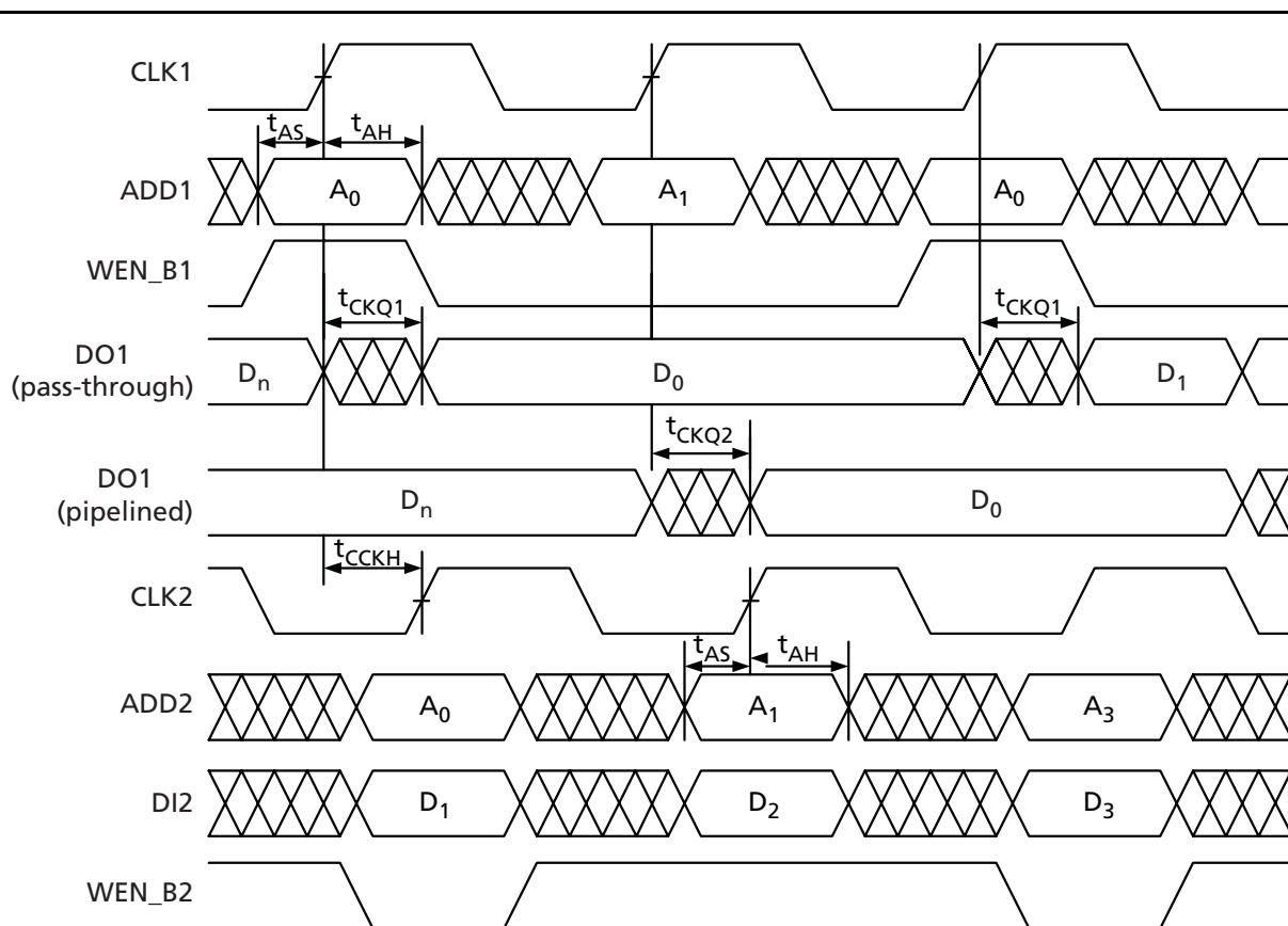
Figure 2-48 • Write Access after Read onto Same Address
