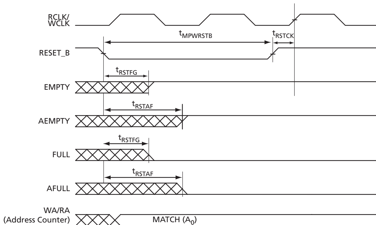
Figure 2-41 • FIFO Reset
