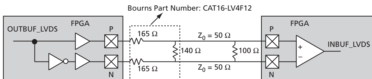
Figure 2-13 • LVDS Circuit Diagram and Board-Level Implementation
