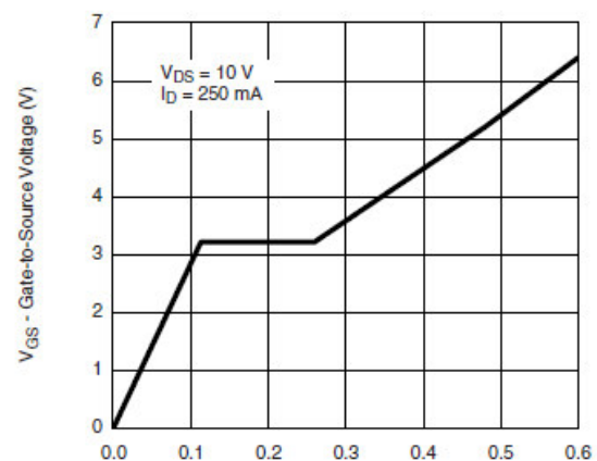
Gate Charge
