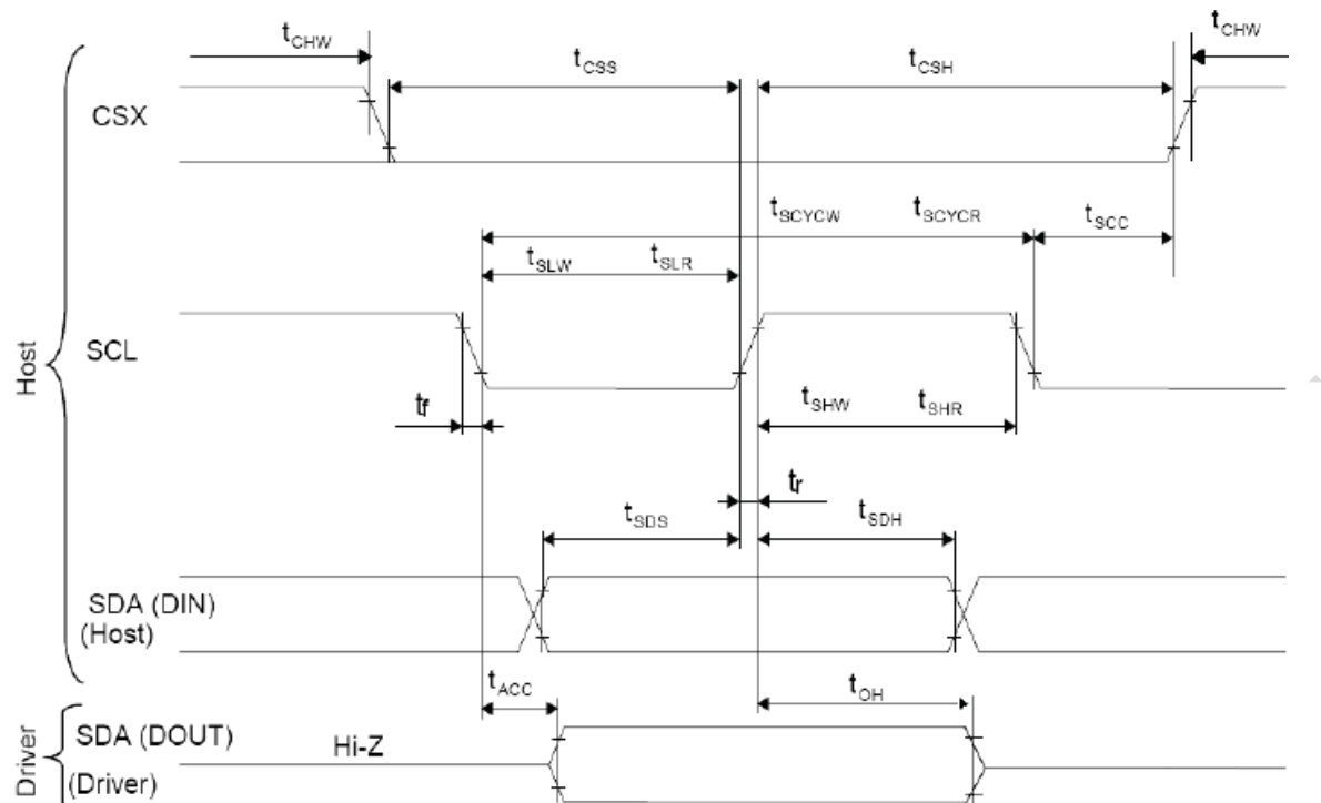
Fig.5-7 AC Characteristics of 3-Wire 9-Bit Serial Interface timing
