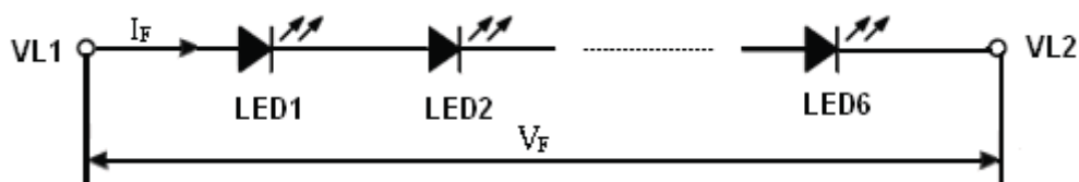
Figure 4.2 LED connection of backlight
