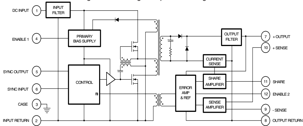
AFL27003R3S Circuit Description Figure I. AFL Single Output Block Diagram
