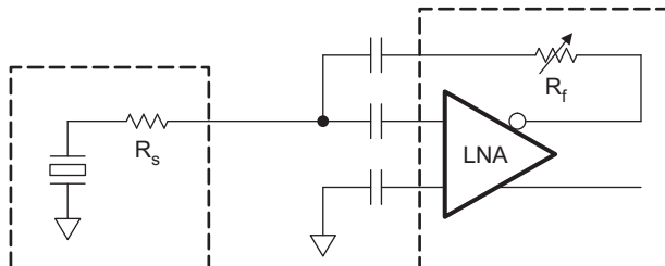
(b) Active Termination
