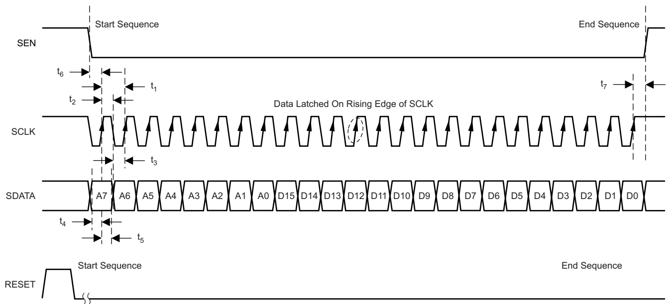
Figure 84. SPI Timing
