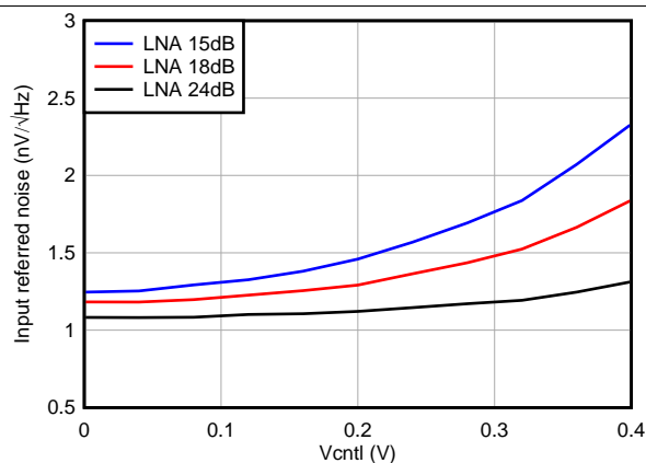
Figure 23. IRN, PGA = 24 dB and Low-Power Mode
