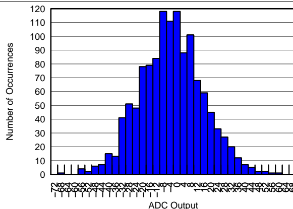
Figure 7. Output Offset Histogram, V_{\text{CNTL}} = 0 V (1247 Channels)
