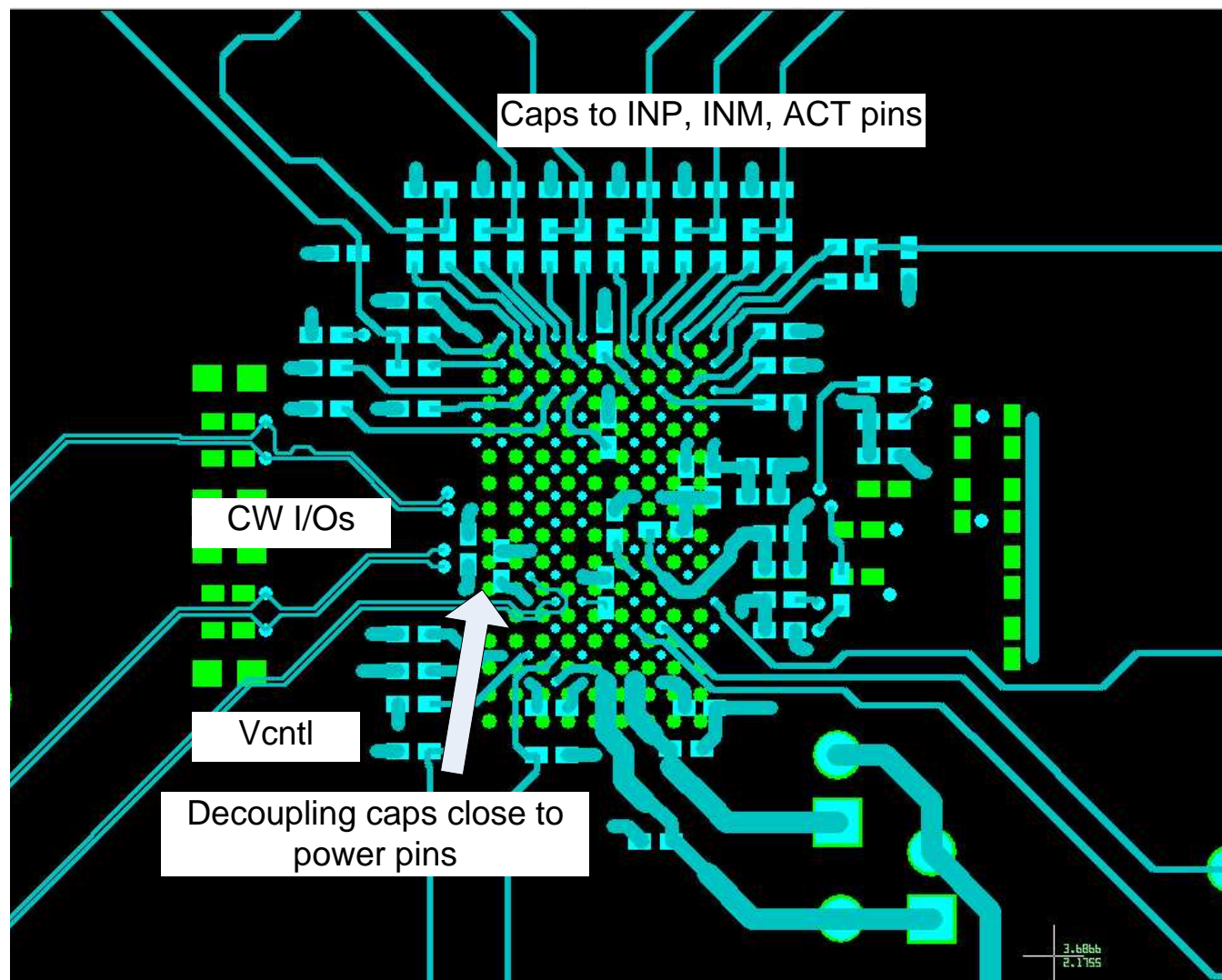
Figure 112. Layout Example
