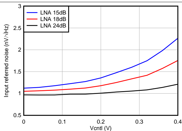
Figure 21. IRN, PGA = 24 dB and Medium-Power Mode
