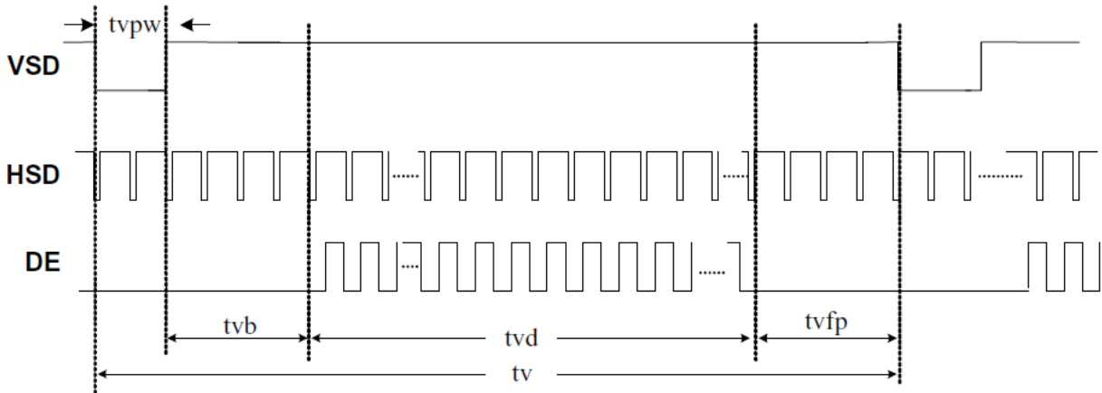
Vertical timing
