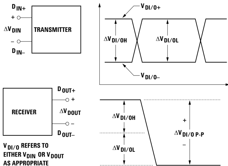
Figure 8. Differential signals.
