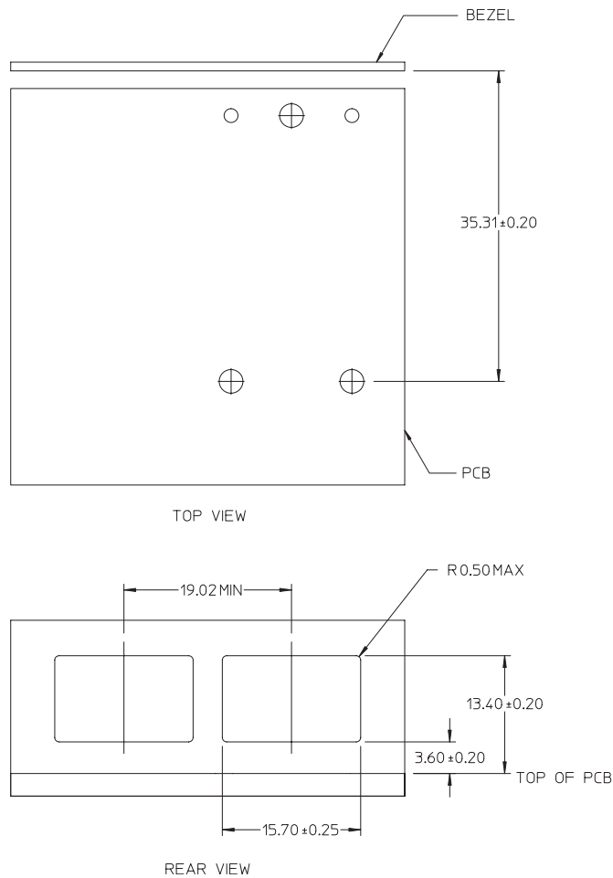
Figure 18. Host Frontplate Layout (dimensions in mm)
