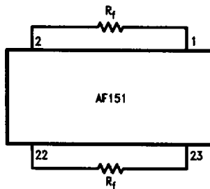
FIGURE 2. Frequency Tuning
