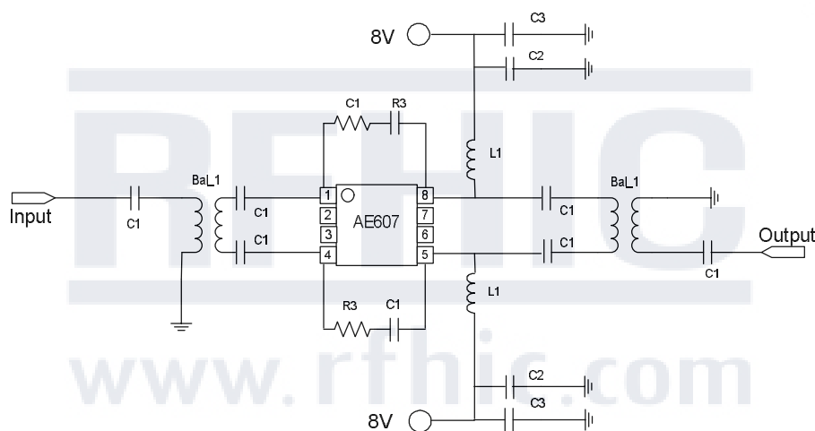
Application Circuit @ 30~1000MHz
