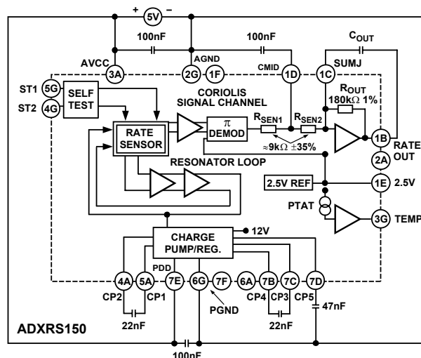
Figure 22. Block Diagram with External Components
