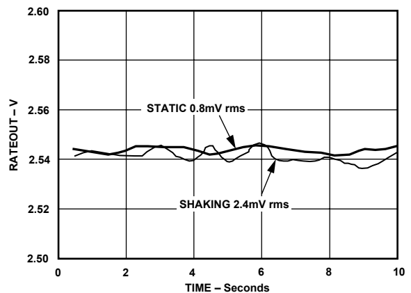
Figure 25. Random Vibration (Lateral) 10 kHz to 20 kHz at 0.01 \text{ g}/\sqrt{\text{Hz}} with 60 Hz Sampling and 0.5 Sec Averaging
