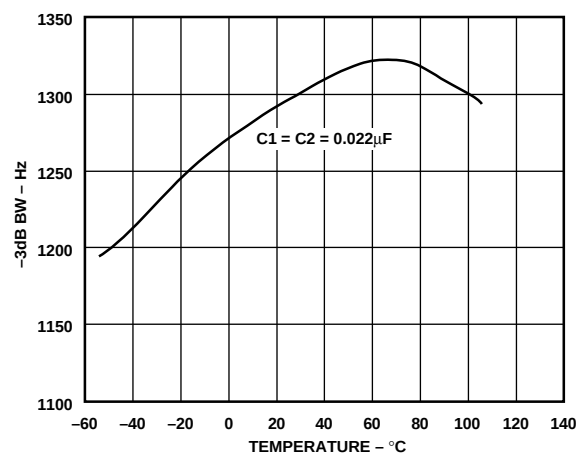
Figure 6. -3 dB Bandwidth vs. Temperature at V_{PR}
