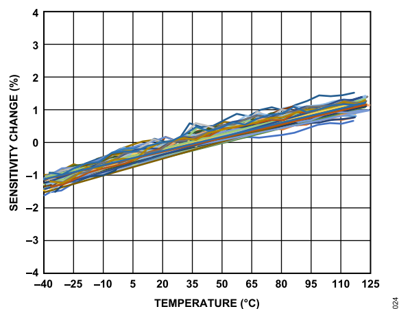
Figure 24. Z-Axis Sensitivity Change vs. Temperature at 25°C, V_S = 3.3\text{ V}
