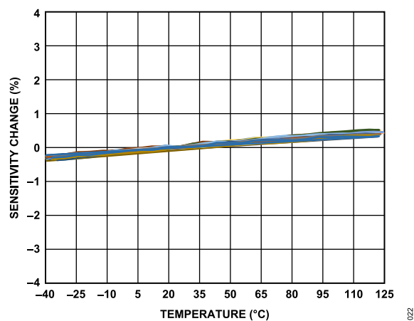
Figure 22. X-Axis Sensitivity Change vs. Temperature at 25°C, V_S = 3.3\text{ V}
