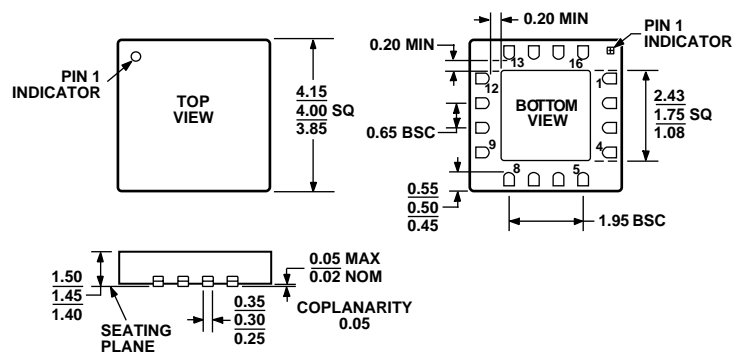
Figure 33. 16-Lead Lead Frame Chip Scale Package [LFCSP_LQ] 4 mm x 4 mm Body, Thick Quad (CP-16-5) Dimensions shown in millimeters
