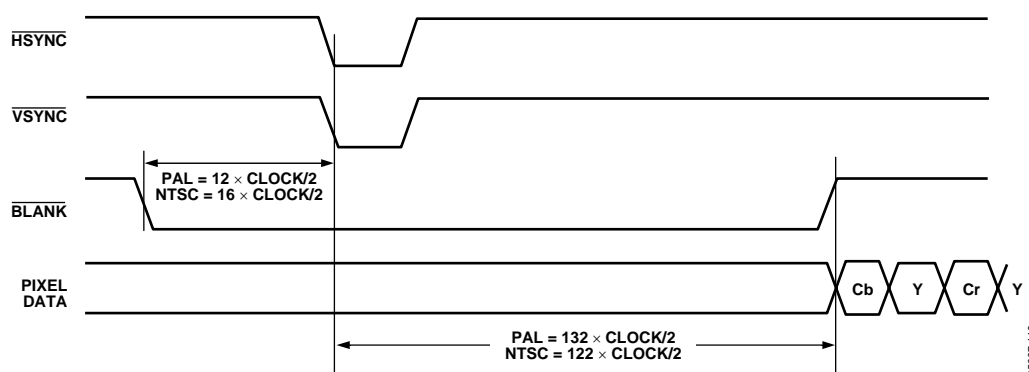
Figure 118. SD Timing Mode 2 Even-to-Odd Field Transition Master/Slave
