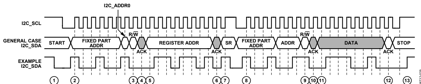
Figure 30. I²C Read Diagram
