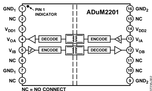
Figure 2. ADuM2201
