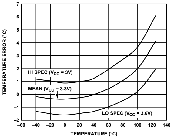
Figure 8. Remote Temperature Error
