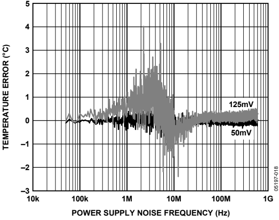
Figure 14. Remote Temperature Error vs. Power Supply Noise
