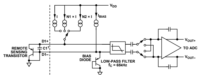
Figure 16. Signal Conditioning for Remote Diode Temperature Sensors
