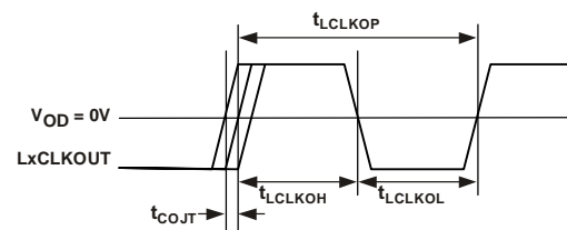
Figure 15. Link Ports—Output Clock
