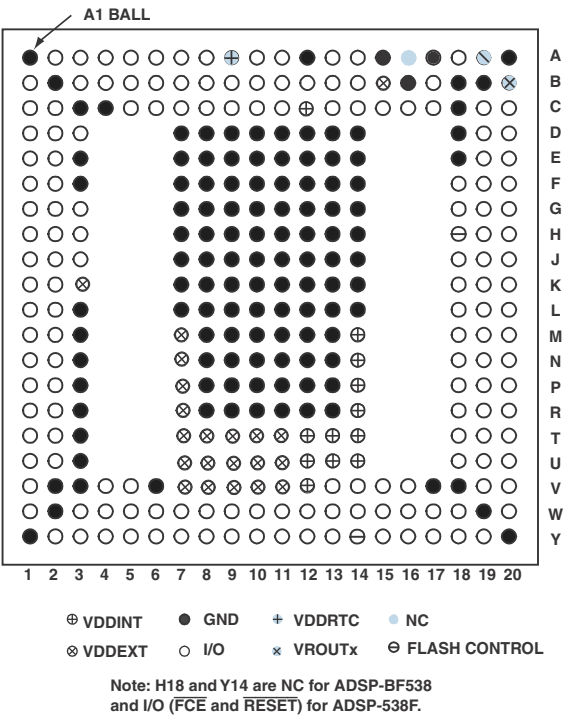
Figure 56. 316-Ball CSP_BGA Ball Assignment (Top View)
