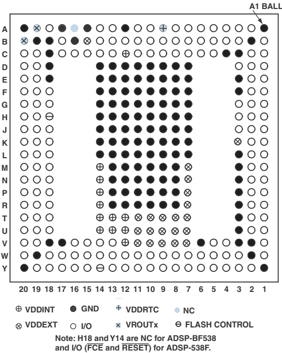
Figure 57. 316-Ball CSP_BGA Ball Assignment (Bottom View)
