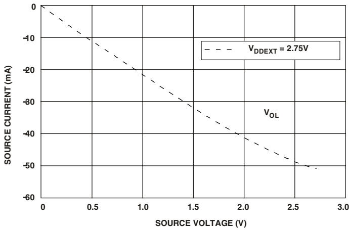
Figure 41. Drive Current E (Low V_{DDEXT} )
