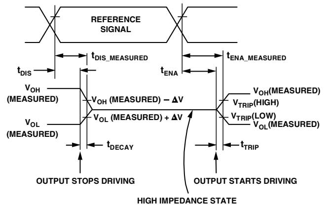
Figure 44. Output Enable/Disable
