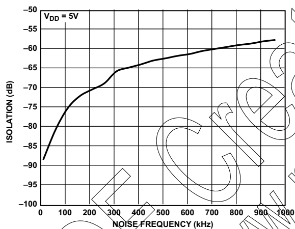
Figure 51. Channel-to-Channel Isolation
