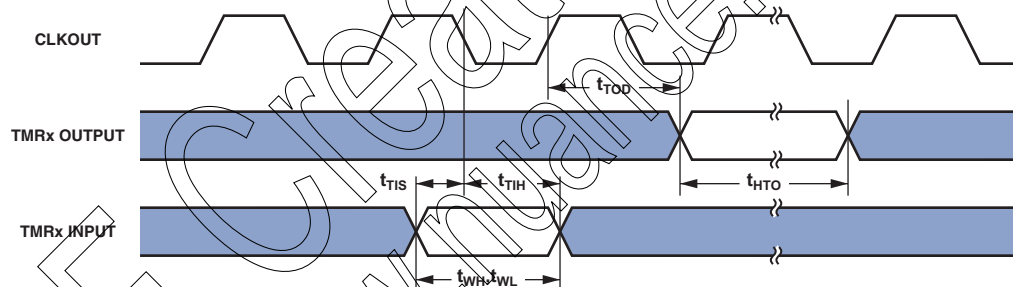
Figure 26. Timer Cycle Timing
