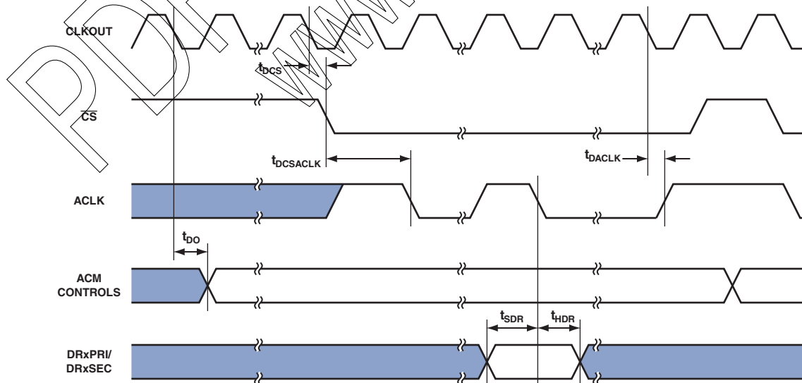
Figure 30. ACM Timing
