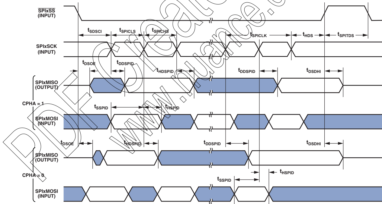
Figure 24. Serial Peripheral Interface (SPI) Port—Slave Timing
