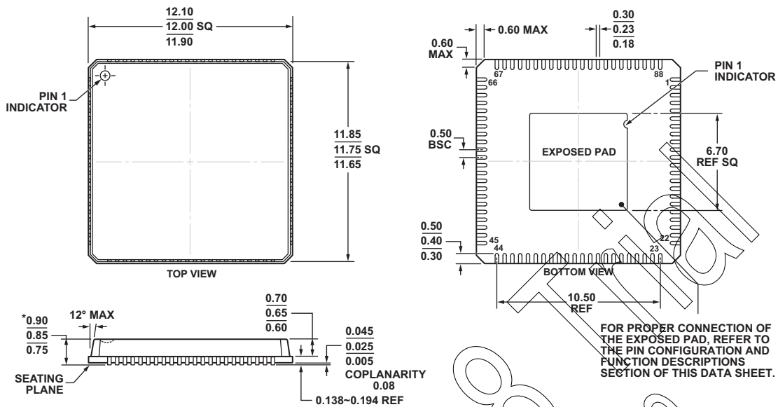
Figure 94. 88-Lead Lead Frame Chip Scale Package (LFCSP_VQ1) 1
