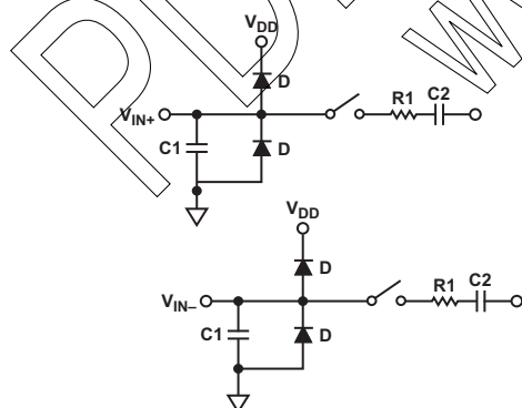
Figure 64. Equivalent Analog Input Circuit, Conversion Phase—Switches Open, Track Phase—Switches Closed
