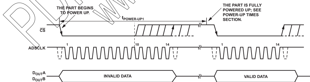
Figure 82. Exiting Partial Power-Down Mode
