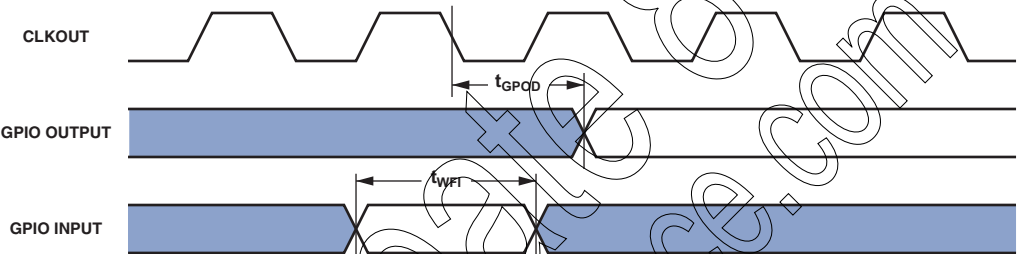
Figure 25. General-Purpose Port Timing
