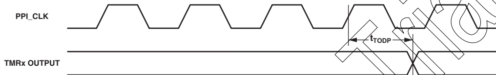
Figure 27. Timer Clock Timing
