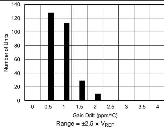
Figure 39. Typical Histogram for Gain Error Drift
