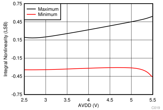
Figure 10. INL vs AVDD
