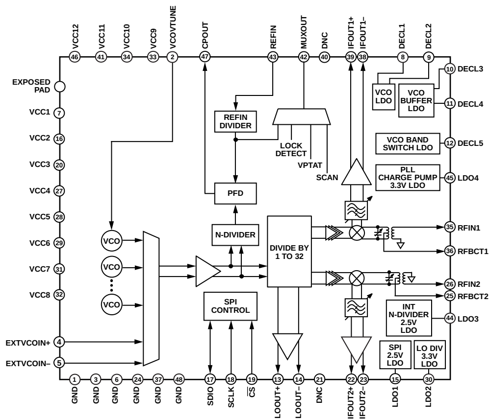
Figure 110. Simplified Schematic
