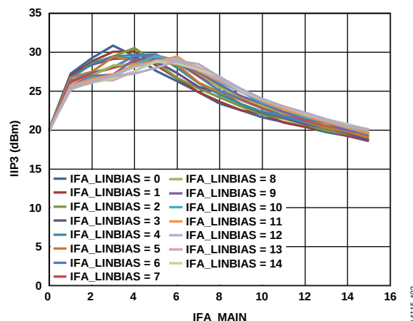
Figure 116. IIP3 vs. Main Bias (IFA_MAINBIAS) and Linearity Bias (IFA_LINBIAS) Level at IF Frequency = 150 MHz
