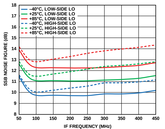
Figure 21. SSB Noise Figure vs. IF Frequency for Three Temperatures
