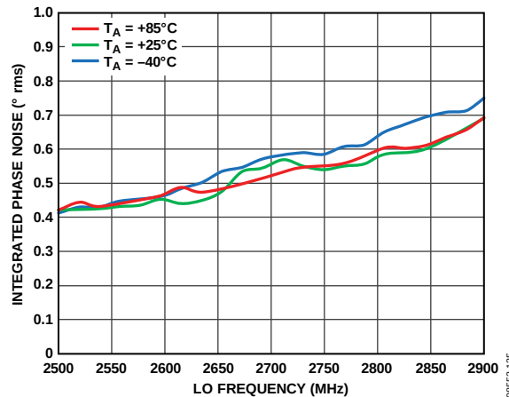
Figure 35. Integrated Phase Noise vs. LO Frequency
