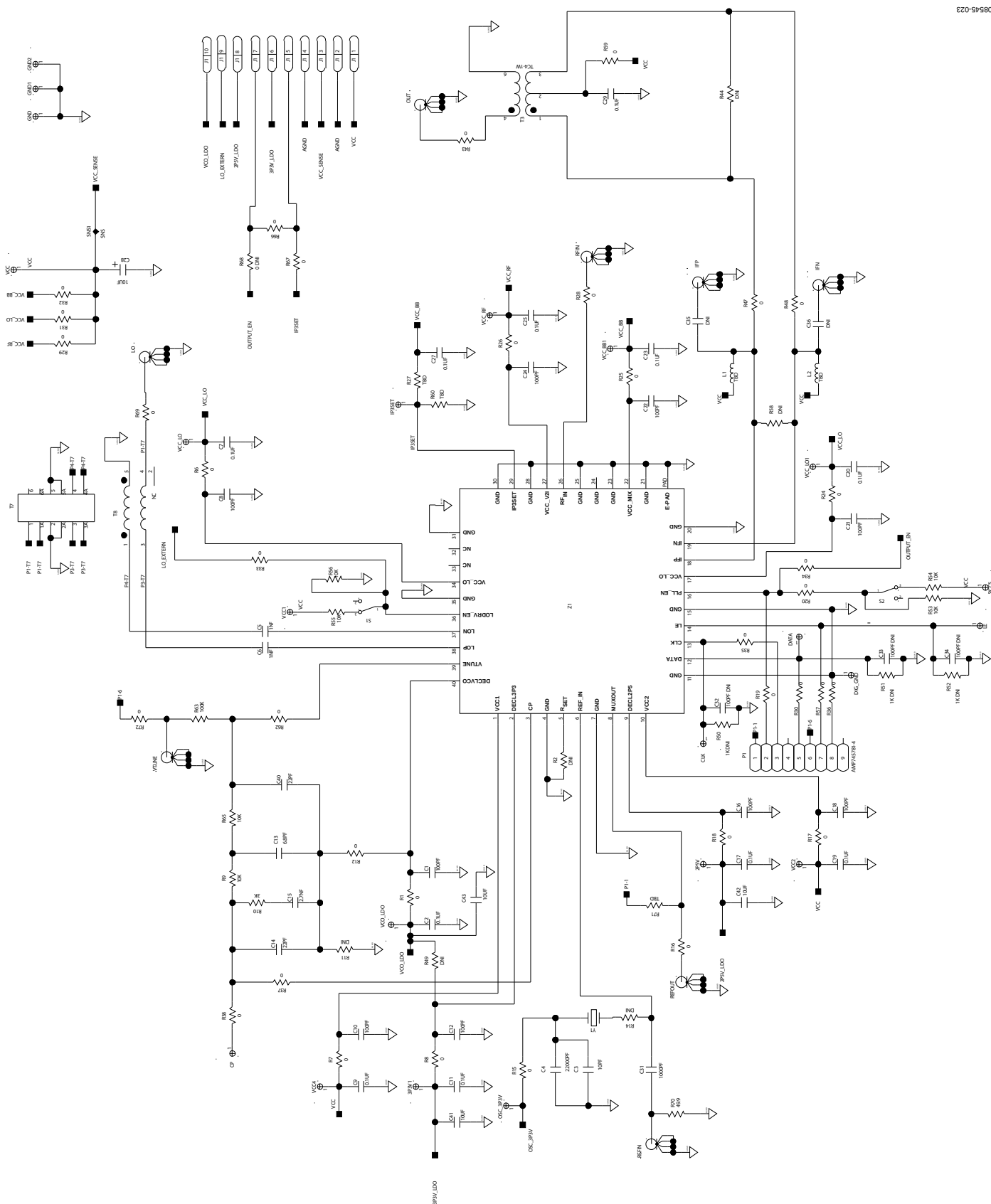
Figure 50. Evaluation Board Schematic
