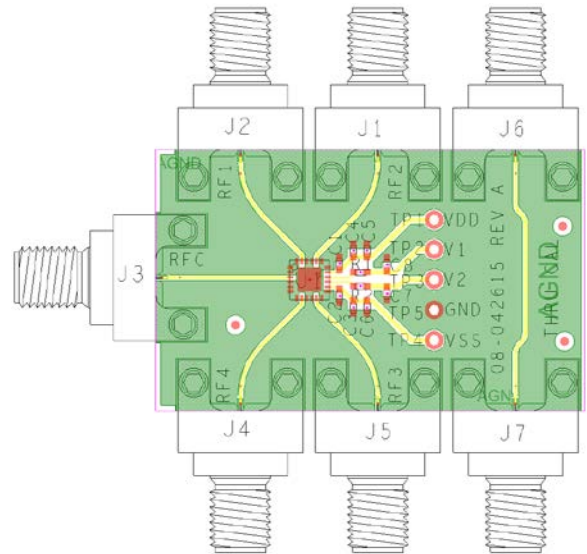
Figure 24. Evaluation Board Component Placement
