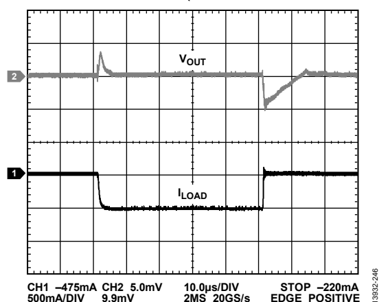
Figure 46. Output Transient Response, C_{OUT} = 4.7 \mu F , V_{OUT} = -1.2 V
