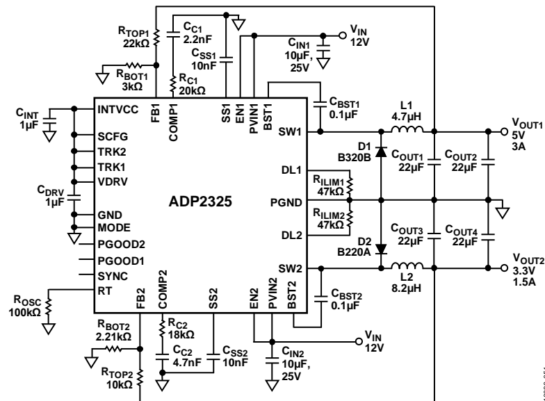
Figure 55. Using an External Diode Application, V_{IN1} = V_{IN2} = 12\text{V} , V_{OUT1} = 5\text{V} , I_{OUT1} = 3\text{A} , V_{OUT2} = 3.3\text{V} , I_{OUT2} = 1.5\text{A} , f_{SW} = 600\text{kHz}
