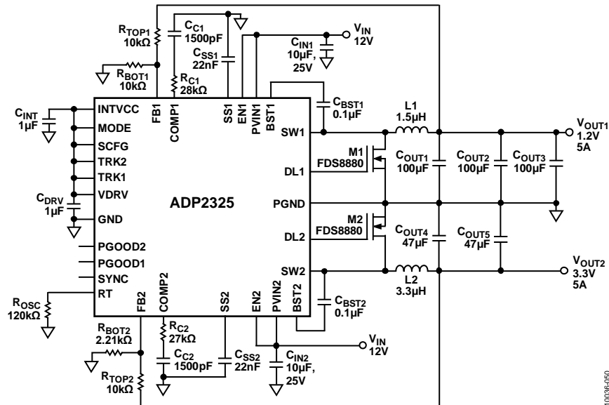
Figure 54. Using an External MOSFET Application, V_{IN1} = V_{IN2} = 12\text{V} , V_{OUT1} = 1.2\text{V} , I_{OUT1} = 5\text{A} , V_{OUT2} = 3.3\text{V} , I_{OUT2} = 5\text{A} , f_{SW} = 500\text{kHz}
