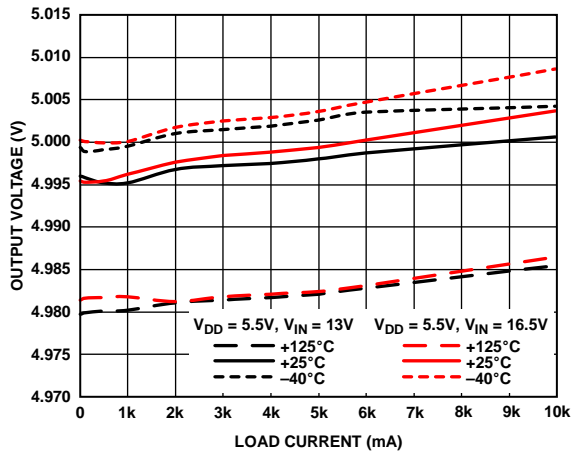
Figure 18. Output Voltage Accuracy—600 kHz, V_{OUT} = 5\text{ V}
