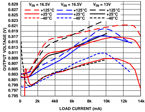
Figure 16. Output Voltage Accuracy—600 kHz, V_{OUT} = 0.8\text{ V}
