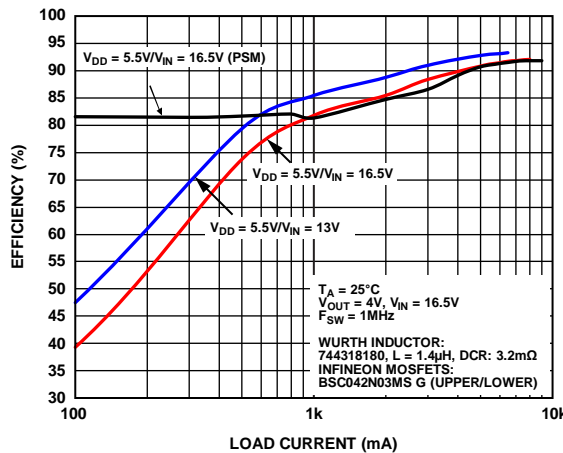
Figure 12. Efficiency—1.0 MHz, V_{OUT} = 4 V
