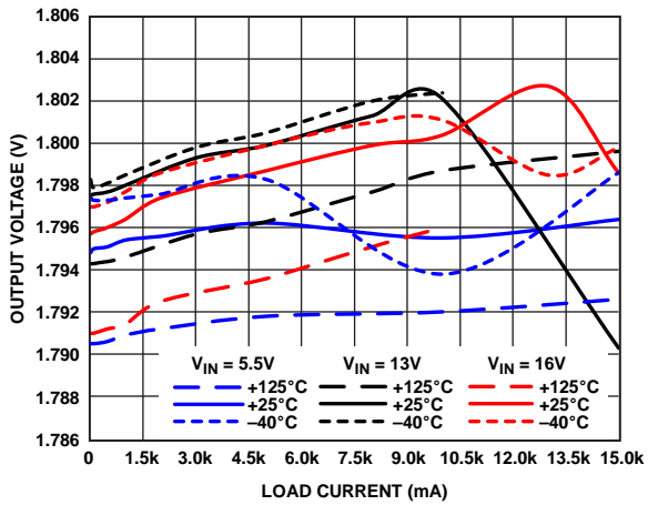
Figure 17. Output Voltage Accuracy—600 kHz, V_{OUT} = 1.8\text{ V}
