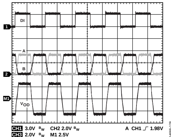
Figure 23. Driver Propagation Delay (Oscilloscope Plot), Data Rate = 500 kbps, 500 kbps Models
