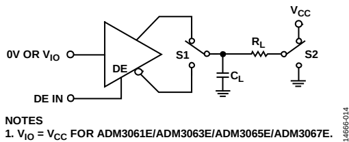
Figure 39. Driver Enable/Disable
