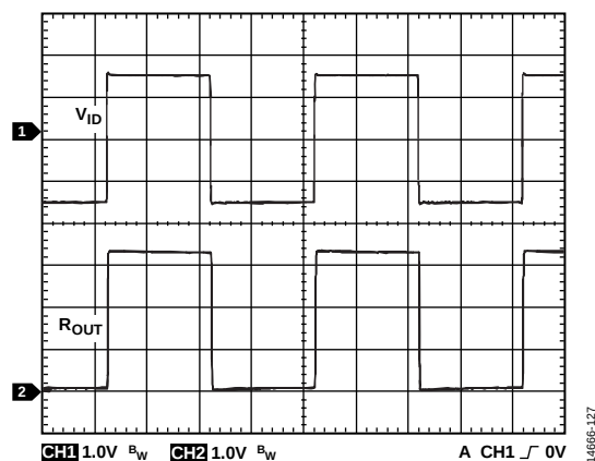
Figure 22. Receiver Propagation Delay (Oscilloscope Plot), Data Rate = 500 kbps, V_D \geq 1.5\text{ V}
