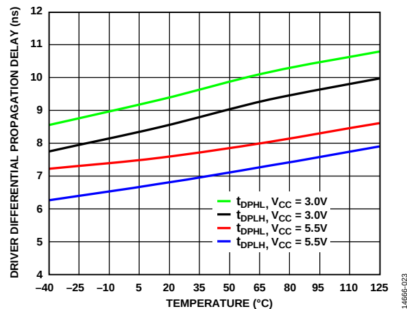
Figure 24. Driver Differential Propagation Delay vs. Temperature, 50 Mbps Models
