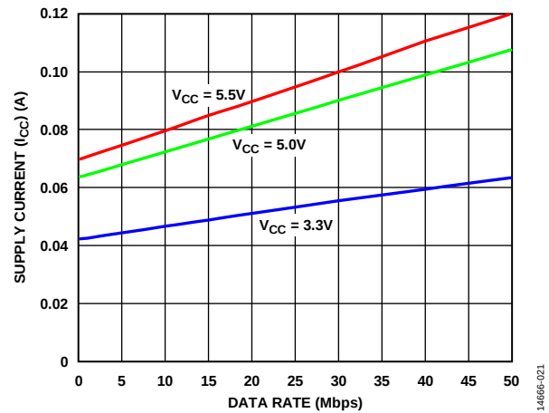
Figure 16. Supply Current ( I_{CC} ) vs. Data Rate with 54\Omega Load Resistance, 50 Mbps Models
