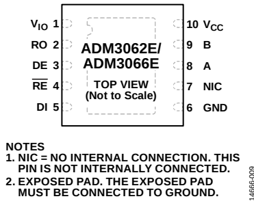
Figure 10. ADM3062E/ADM3066E 10-Lead LFCSP Pin Configuration
