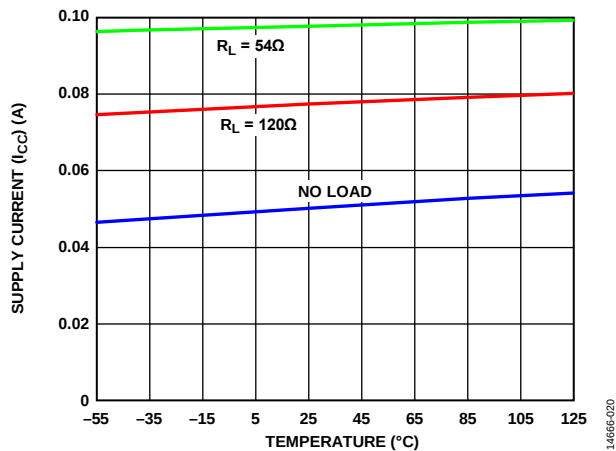
Figure 15. Supply Current ( I_{CC} ) vs. Temperature, Data Rate = 50 Mbps, 50 Mbps Models, V_{CC} = 5.0V
