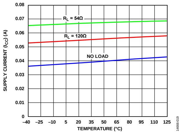
Figure 14. Supply Current ( I_{CC} ) vs. Temperature, Data Rate = 50 Mbps, 50 Mbps Models, V_{CC} = 3.3V
