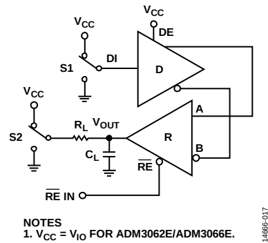
Figure 41. Receiver Enable/Disable from Shutdown
