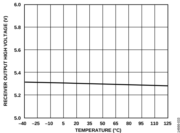
Figure 34. Receiver Output High Voltage vs. Temperature
