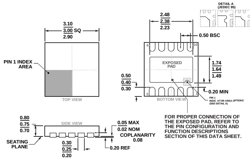
Figure 51. 10-Lead Lead Frame Chip Scale Package [LFCSP] 3 mm x 3 mm Body and 0.75 mm Package Height (CP-10-9) Dimensions shown in millimeters
