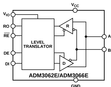
Figure 2. ADM3062E/ADM3066E Functional Block Diagram
