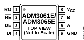
Figure 9. ADM3061E/ADM3065E 8-Lead MSOP Pin Configuration
