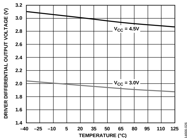
Figure 27. Driver Differential Output Voltage vs. Temperature
