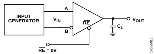
Figure 40. Receiver Propagation Delay/Skew
