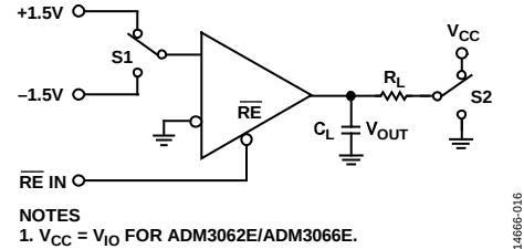
Figure 41. Receiver Enable/Disable from Shutdown
