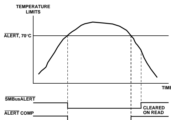
Figure 31. \overline{\text{ALERT}} Comparator and \overline{\text{SMBusALERT}} Outputs
