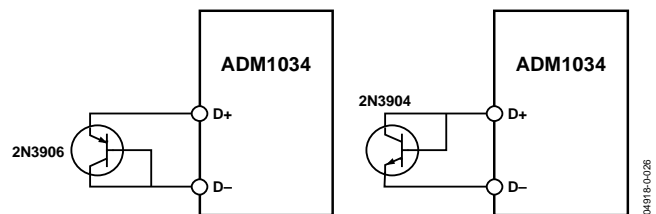
Figure 27. Measuring Temperature by Using Discrete Transistors
