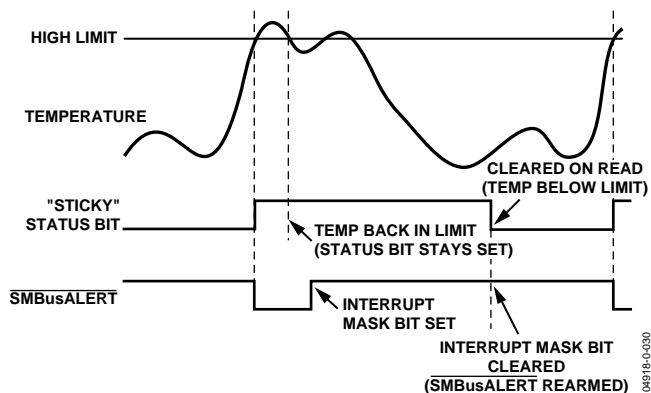
Figure 32. Handling SMBusALERT
