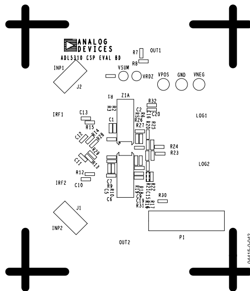
Figure 42. Component-Side Silkscreen
